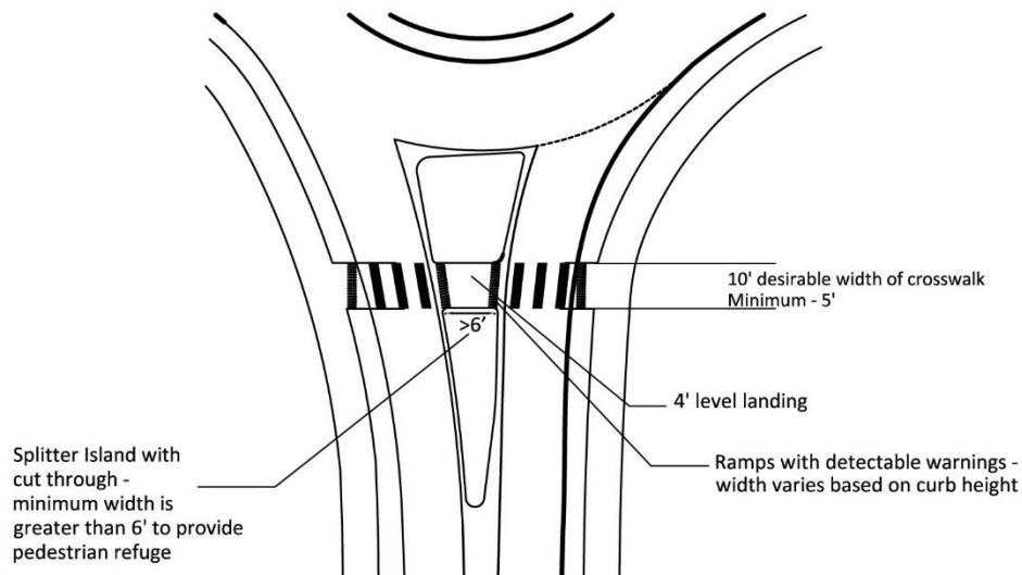
Figure 4-20: Minimum refuge island dimensions for island with ramps
