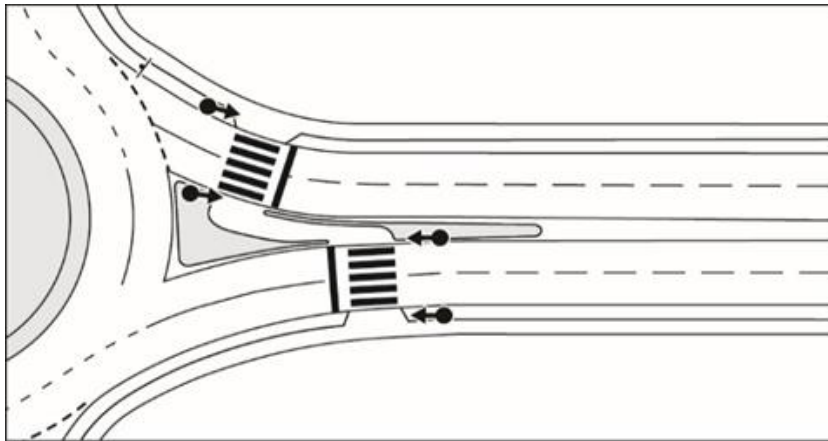
Figure 4-25: Use of side-mounted vehicle displays only at roundabout
