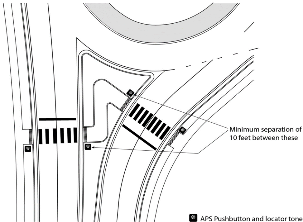
Figure 4-26: Location of Pedestrian Pushbuttons for Zig-Zag Crossing
