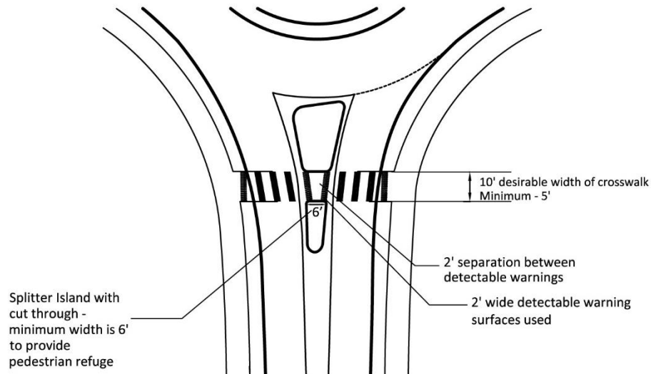
Figure 4-19: Minimum refuge island dimensions for cut-through island
