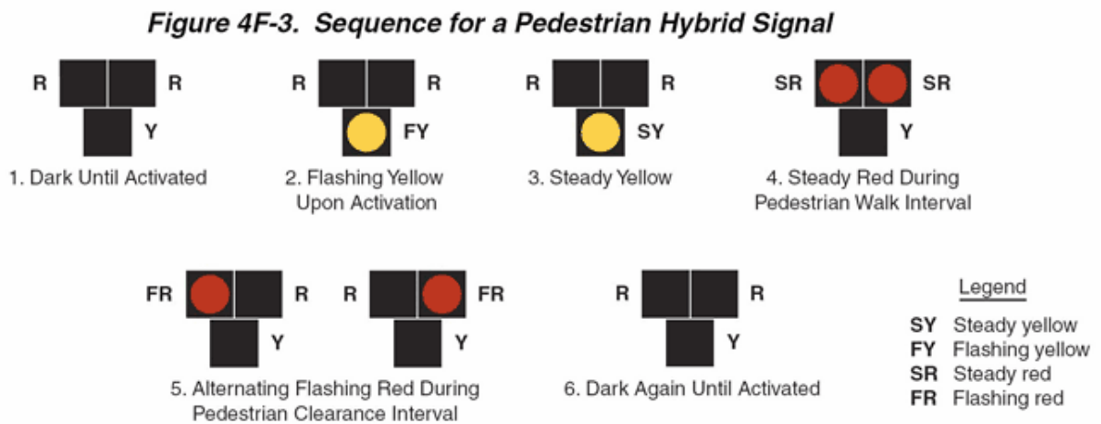
Figure 10-2: PHB Sequence
