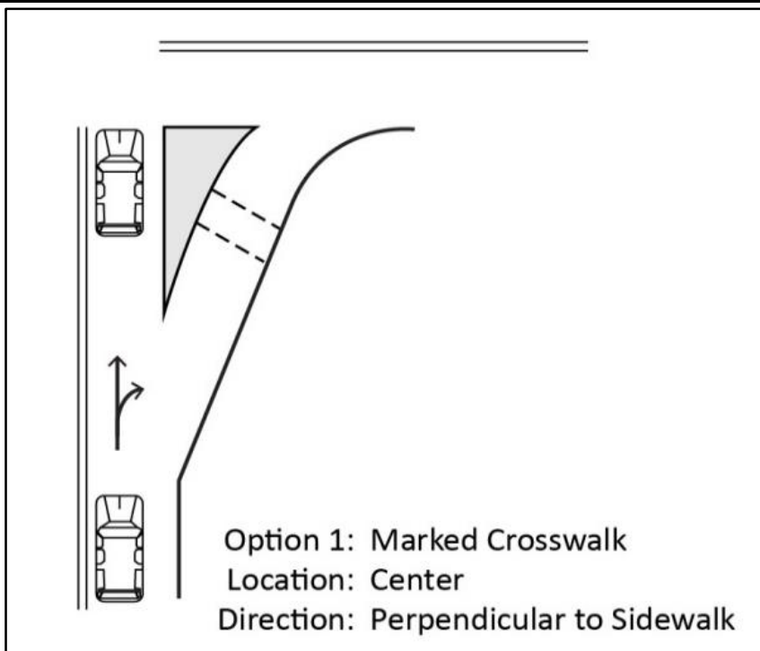
Figure 5-8: Recommended Crosswalk Location and Configuration for CTLs
