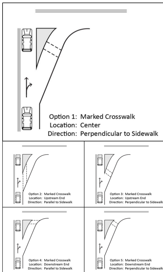
Figure 5-7: CTL crosswalk location options (adapted from (6))
