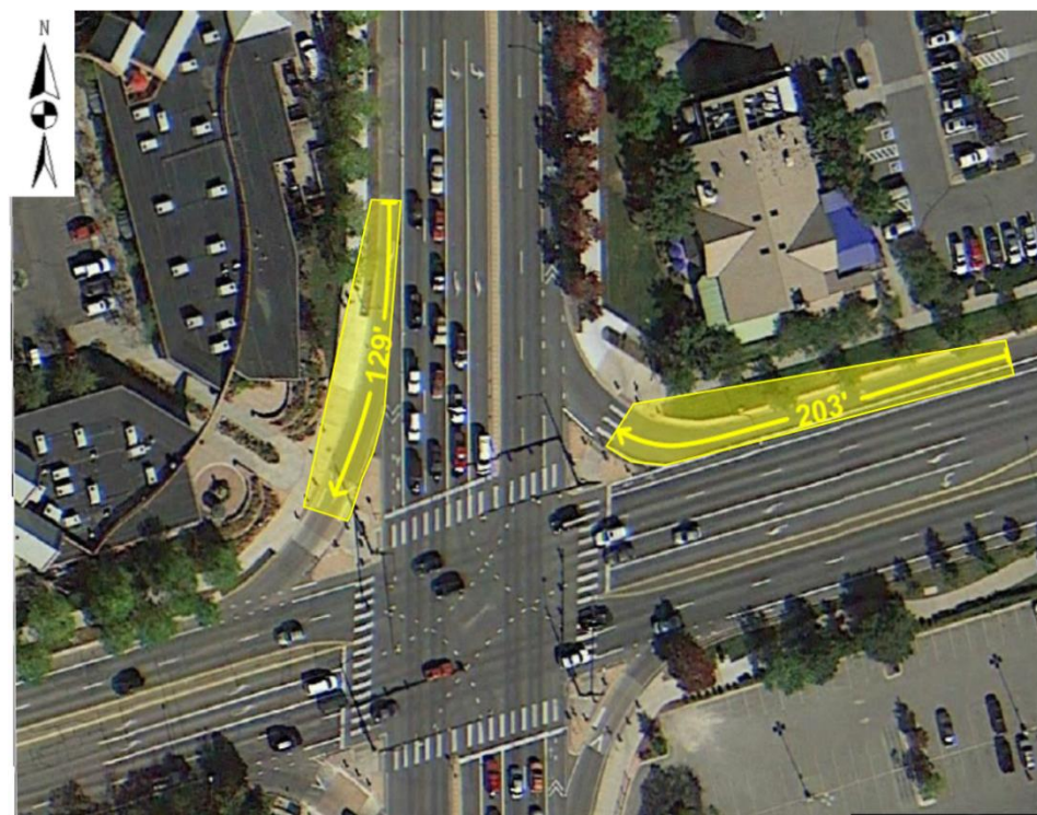
Figure 7-6: Illustration of Sight Distance for CTL with and without raised crosswalk
