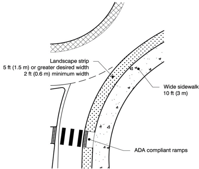
Figure 4-6: Roundabout with landscape buffer following roadway curvature
