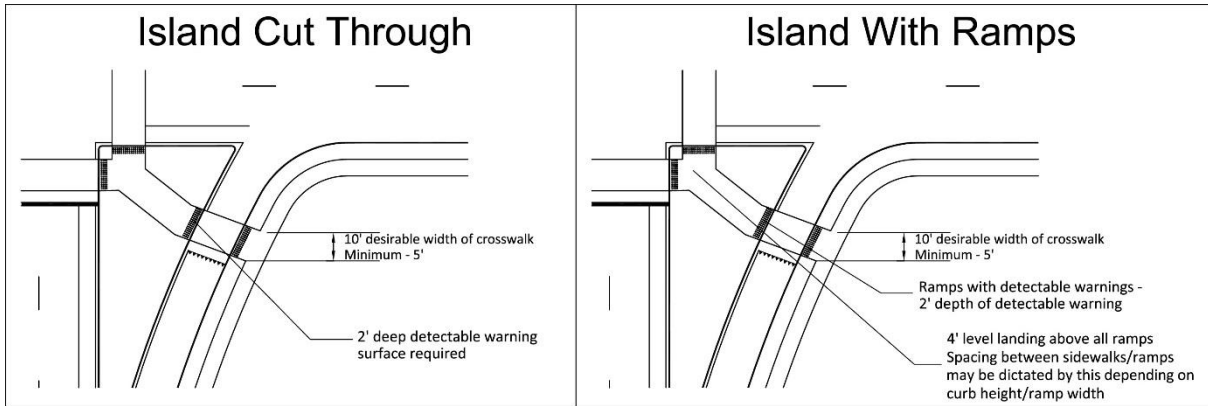
Figure 5-4: Minimum CTL island and Crosswalk dimensions
