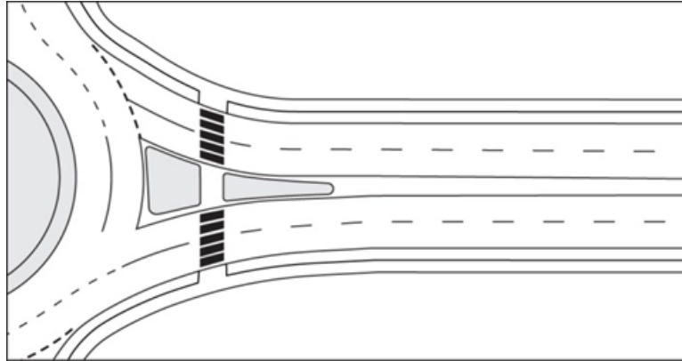
Figure 4-2: Entry and exit crosswalks same distance from roundabout with straight alignment
