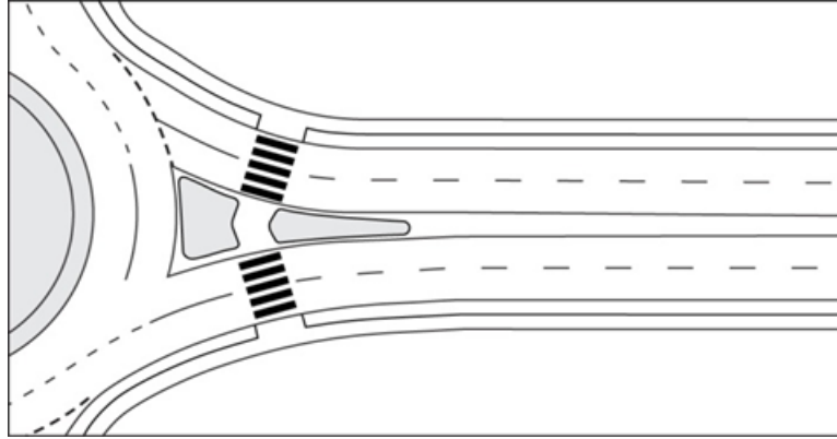
Figure 4-3: Entry and exit crosswalks same distance from roundabout with angled alignment
