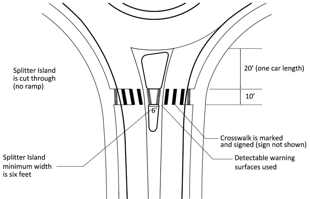
Figure 4-1: Typical crosswalk dimensions and features single lane roundabout
