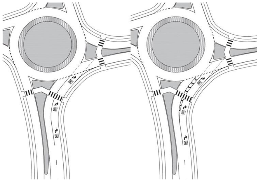
Figure 4-21: Types of non-bypass right-turn lanes at roundabouts
