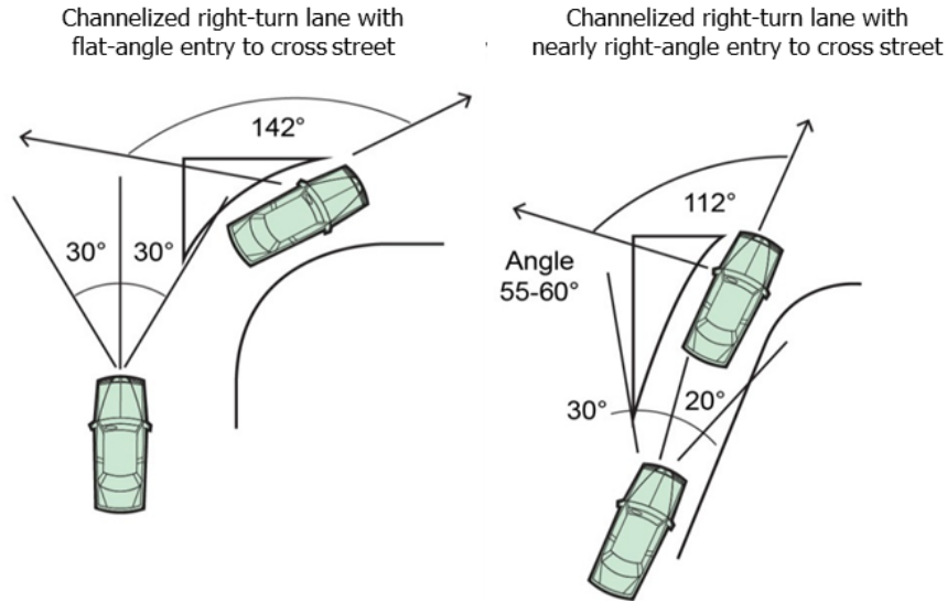
Figure 5-6: Typical CTLs with Differing Entry Angles to the Cross Street
