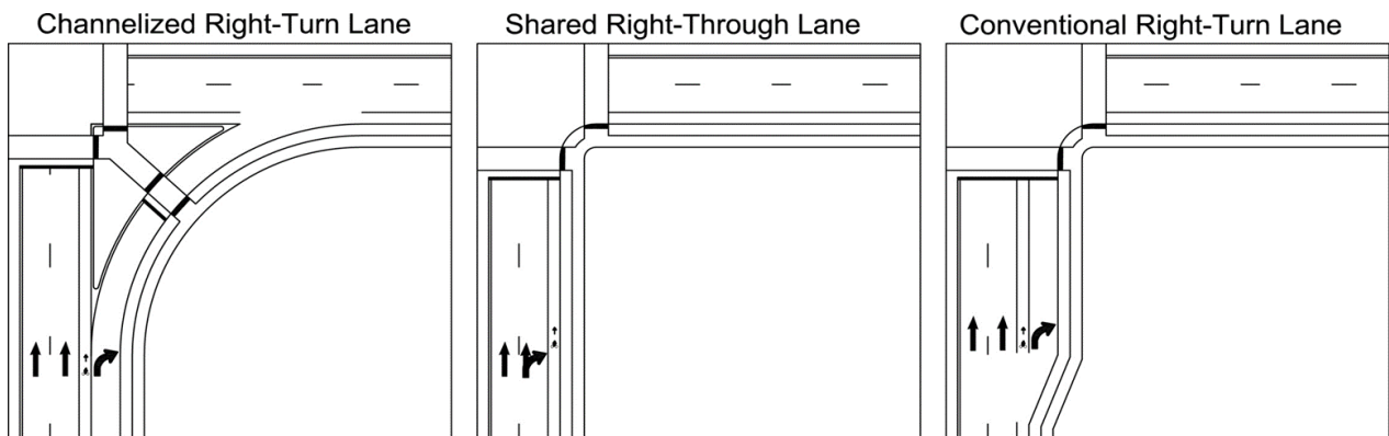
Figure 5-1: Types of Right Turn Lanes
