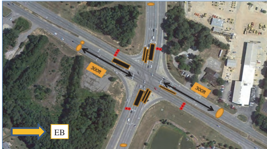
Figure 5-10 Detector configuration of Timber Dr. Intersection on US 70
