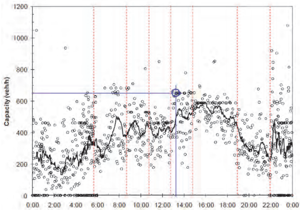
Figure 2-16 Estimated Capacity
