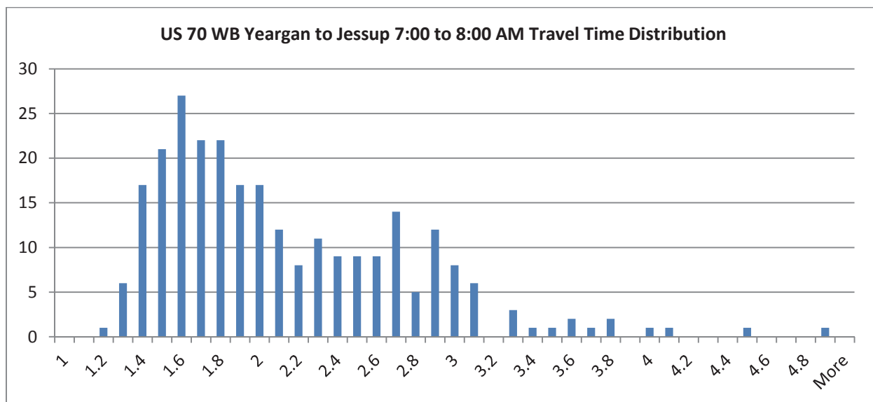
Figure 5-8 U.S. 70 Westbound Travel Time Distribution (7AM to 8AM)
