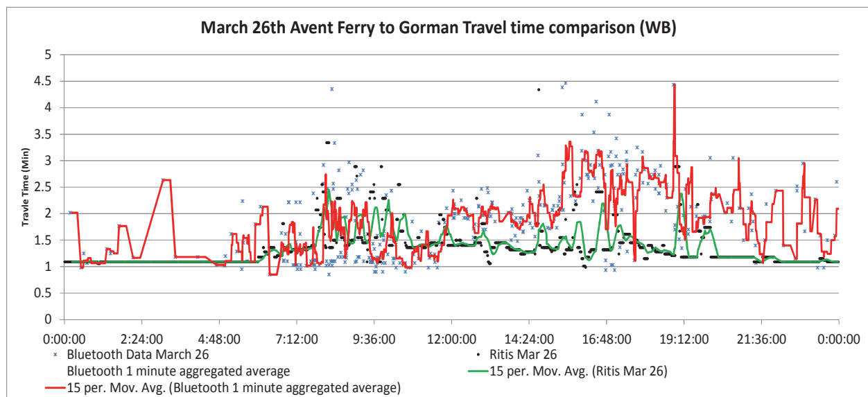
Figure 9-5 WB Travel Time Comparison (TMC 125+14768)
