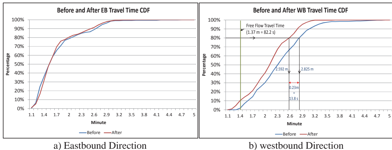
Figure 7-6 Directional Before and After Travel Time CDF's for 1:30 pm Plan at Site A
