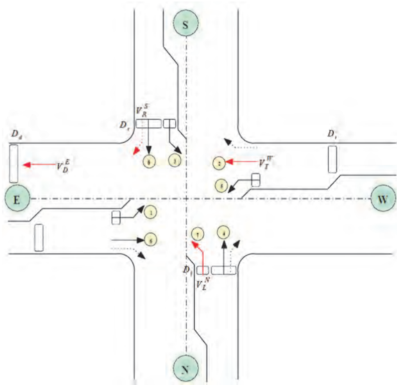
Figure 2-10 SMART-SIGNAL Detector Location Configuration (34)
