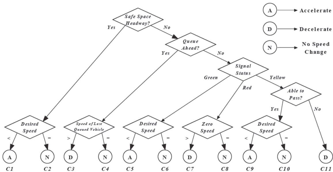
Figure 2-11 SMART-SIGNAL Virtual Vehicle Maneuver Decision Tree (34)
