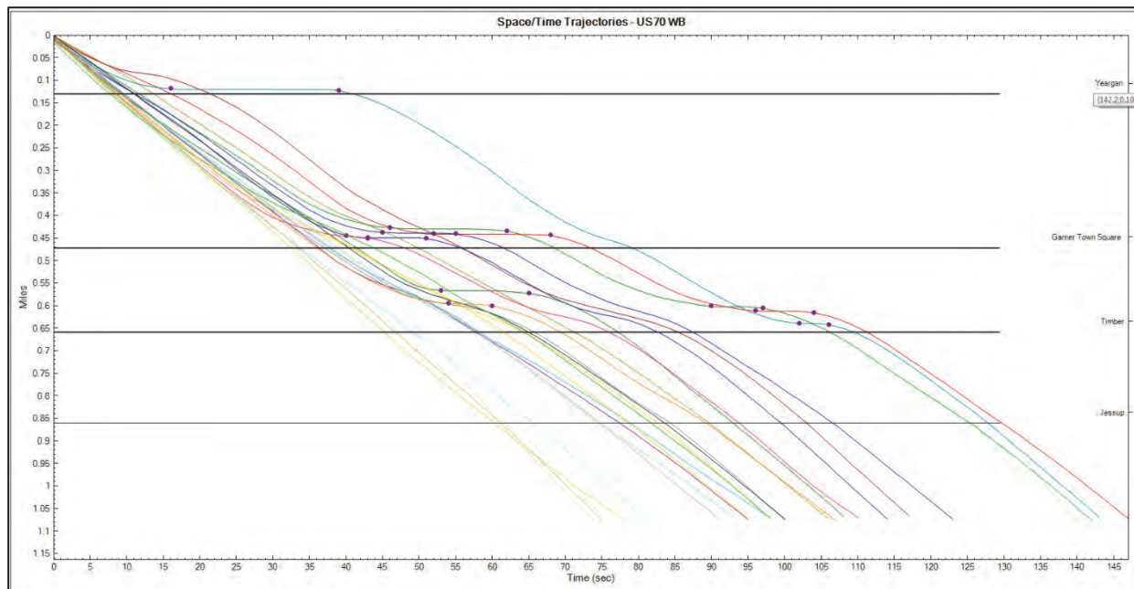
Figure 5-5 U.S. 70 Westbound Corridor Space/Time Trajectories
