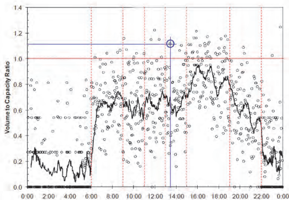
Figure 2-17 Volume to Capacity Ratio Monitoring Results
