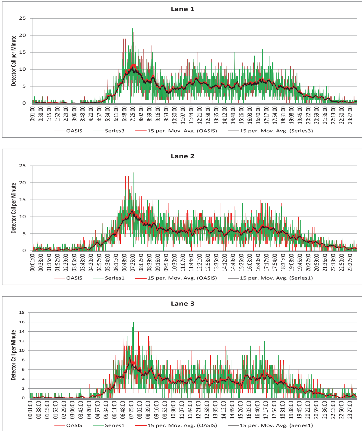
Figure 9-6 OASIS and Sensys Detector Call Comparison
