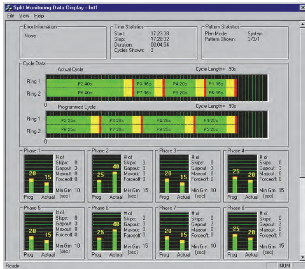
Figure 7-7 ACTRA Split Monitoring Data Display Window
