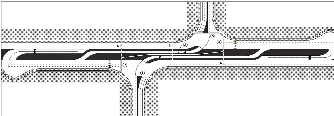
Figure A2. Suggested pedestrian crossing location for reverse offset of minor streets at a superstreet.
