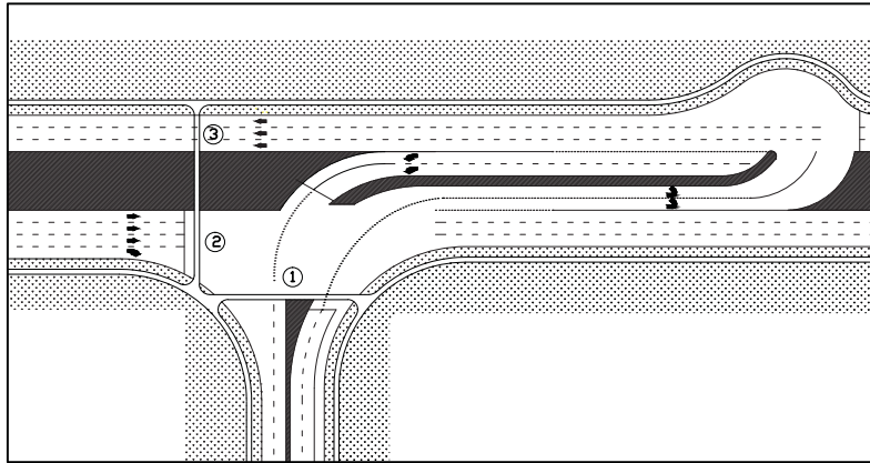
Figure A3. Suggested pedestrian crossing location at a 3-way superstreet intersection.
