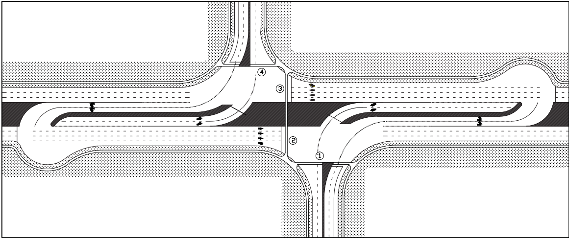
Figure A1. Suggested pedestrian crossing location for offset minor streets at a superstreet.
